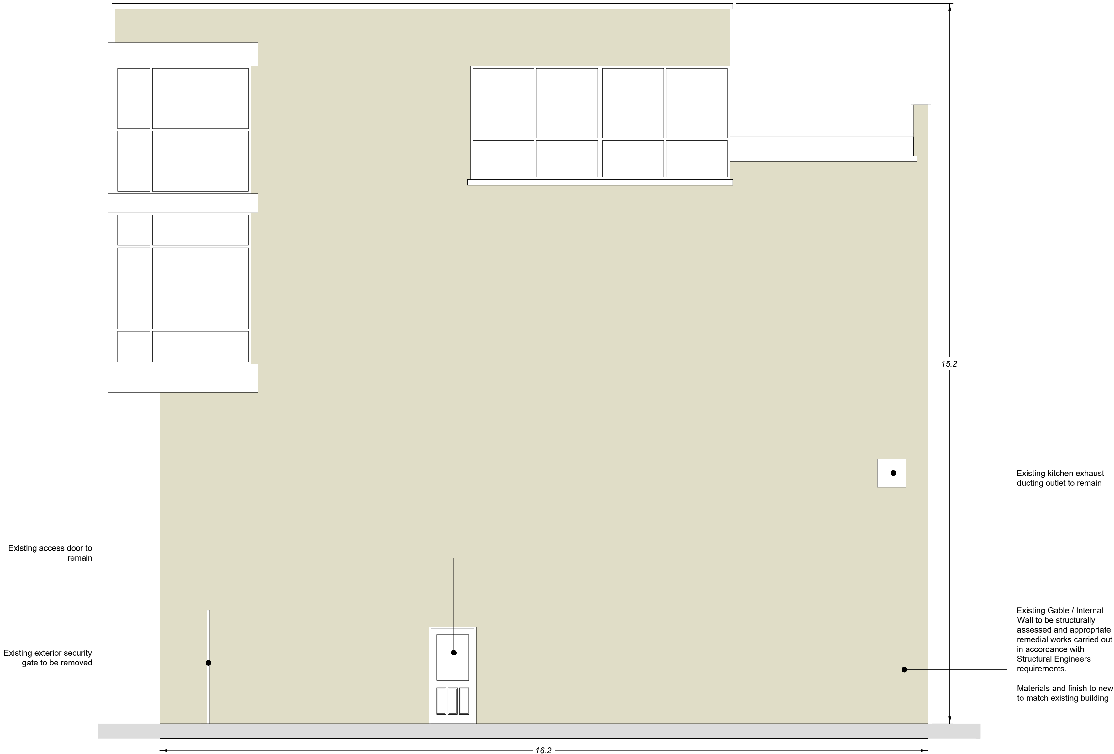
ELEVATION 2-2 SCALE 1:50
